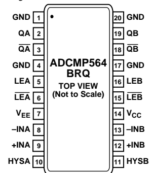
Figure 3. ADCMP564 20-Lead QSOP
