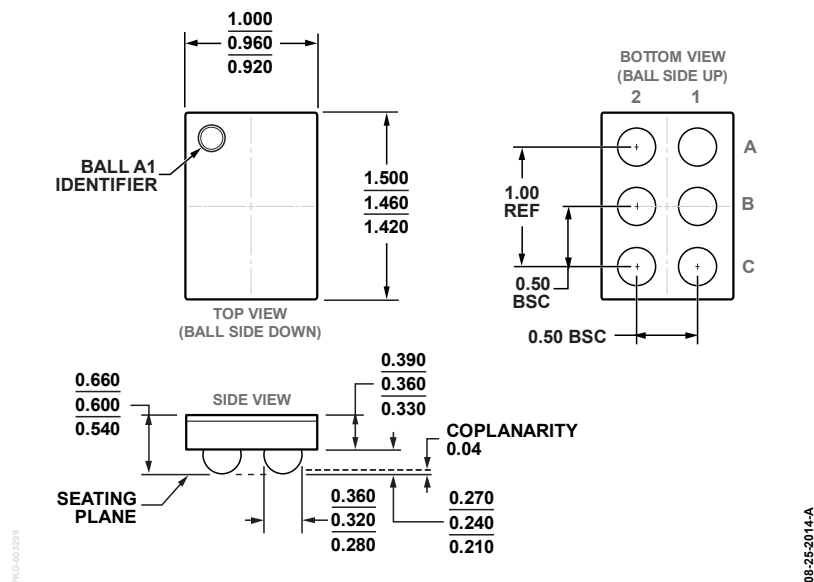
Figure 17. 6-Ball Wafer Level Chip Scale Package [WLCSP] (CB-6-17)
