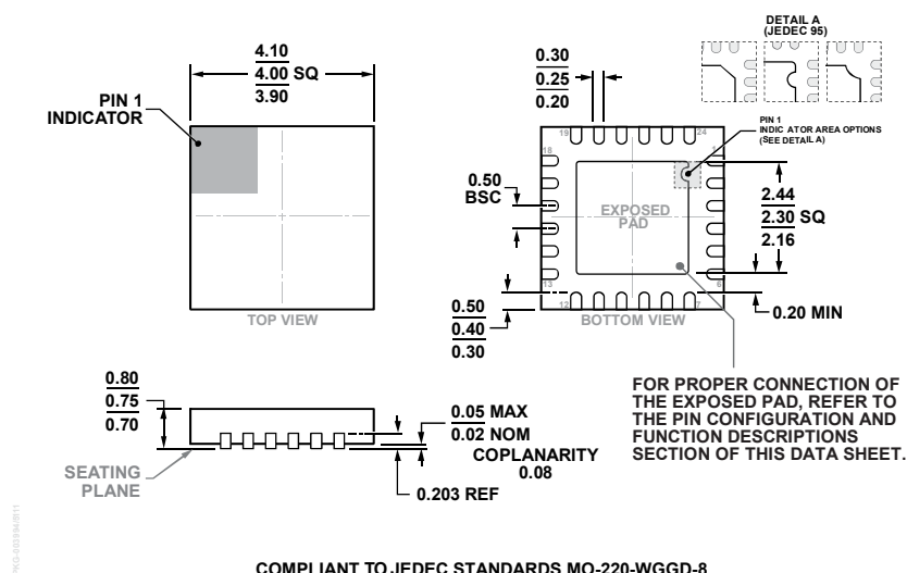
Figure 33. 24-Lead Lead Frame Chip Scale Package [LFCSP] 4 mm × 4 mm Body and 0.75 mm Package Height CP-24-14
