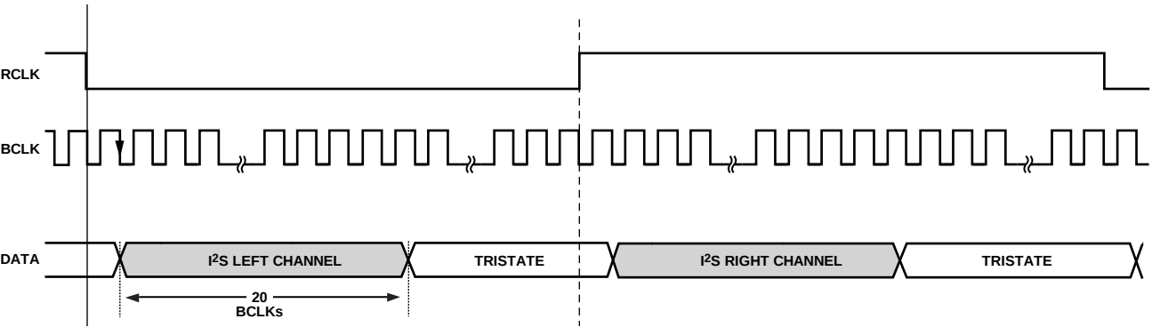
Figure 14. I²S, CONFIG Pin Tied to IOVDD
