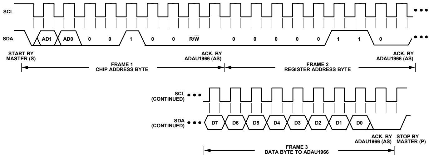
Figure 12. I²C Write Format
