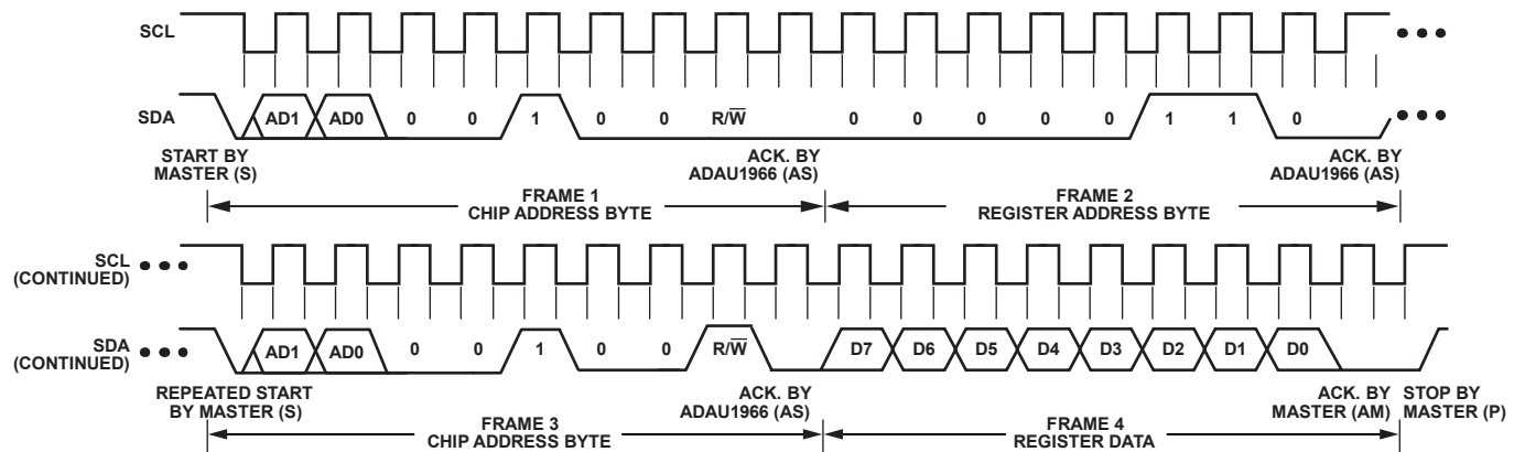
Figure 13. I²C Read Format
