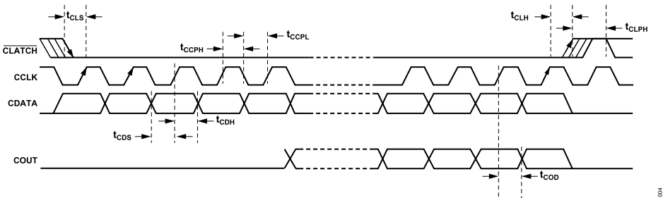
Figure 4. SPI Port Timing
