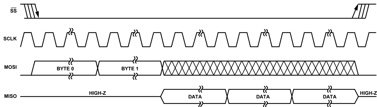
Figure 90. SPI Read from ADAU1772 Clocking (Single-Read Mode)
