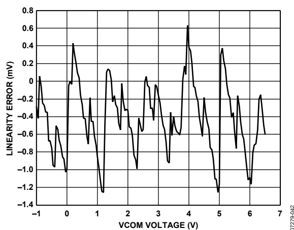
Figure 40. Active Load VCOM Linearity
