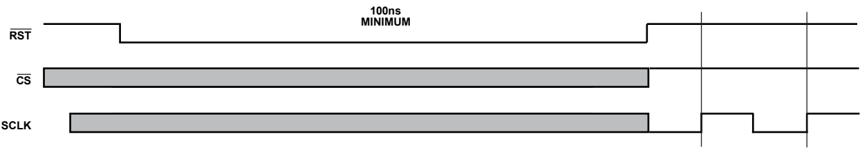
Figure 74. Reset Operation
