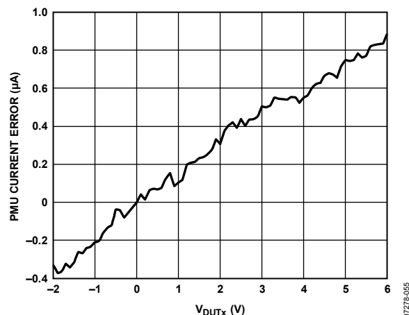
Figure 61. PMU Force Current Range B Output Current Error at 2 mA vs. Output Voltage; Output Voltage Is Pulled Externally
