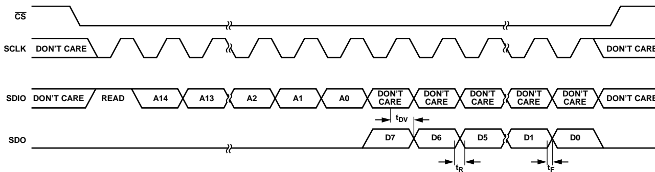
Figure 4. SPI 4-Wire Read Timing Diagram
