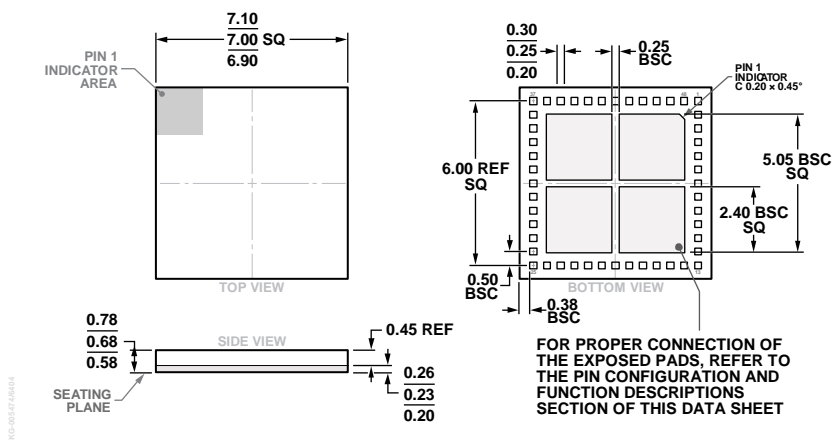
Figure 47. 48-Terminal Land Grid Array [LGA] Package 7 mm × 7 mm Body and 0.68 mm Package Height (CC-48-2)
