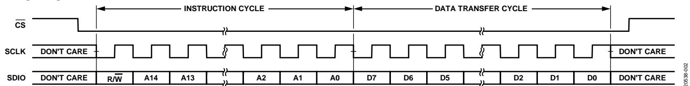
Figure 2. SPI Transaction Structure (MSB First)
