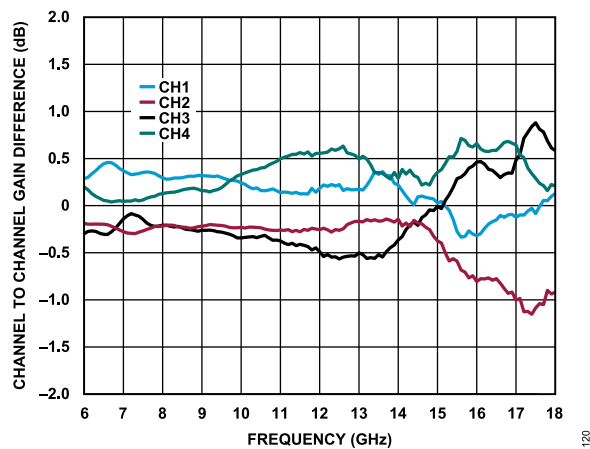
Figure 22. Channel to Channel Gain Difference vs. Frequency, Receive Channel
