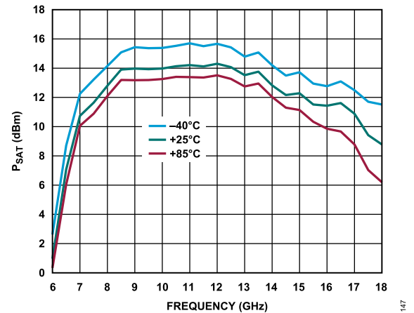
Figure 50. P_{SAT} vs. Frequency, Transmit Channel, Low Bias, Maximum Gain and Phase Set to 45°, All Channels Enabled
