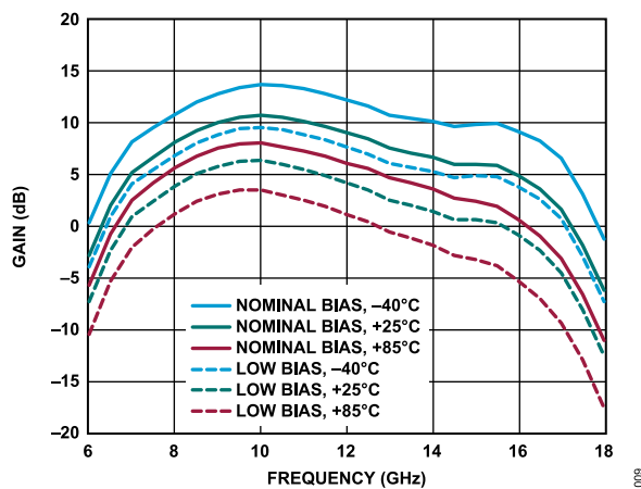
Figure 12. Gain vs. Frequency over Bias and Temperature, Receive Channel
