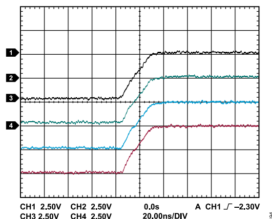
Figure 100. PA_BIAS1, PA_BIAS2, PA_BIAS3, or PA_BIAS4 Rise Time; -10\text{ mA} Load, Measured on P9A of ADAR1000-EVALZ
