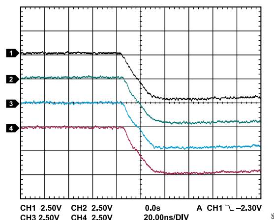
Figure 101. PA_BIAS1, PA_BIAS2, PA_BIAS3, or PA_BIAS4 Fall Time; -10\text{ mA} Load, Measured on P9A of ADAR1000-EVALZ
