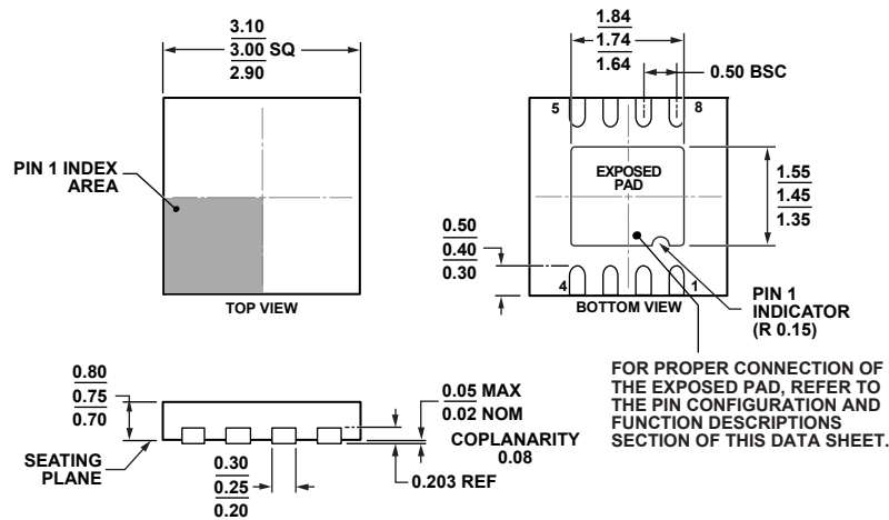
Figure 60. 8-Lead Lead Frame Chip Scale Package [LFCS] 3 mm x 3 mm Body and 0.75 mm Package Height (CP-8-13)
