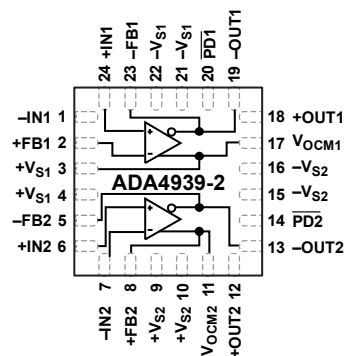
Figure 2. ADA4939-2
