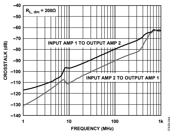
Figure 34. Crosstalk vs. Frequency for ADA4939-2
