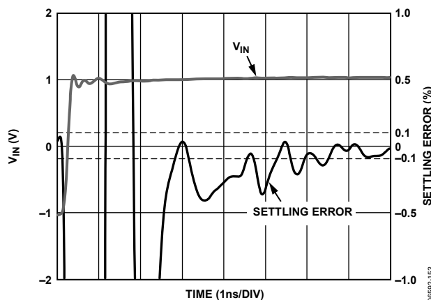
Figure 53. 0.1% Settling Time
