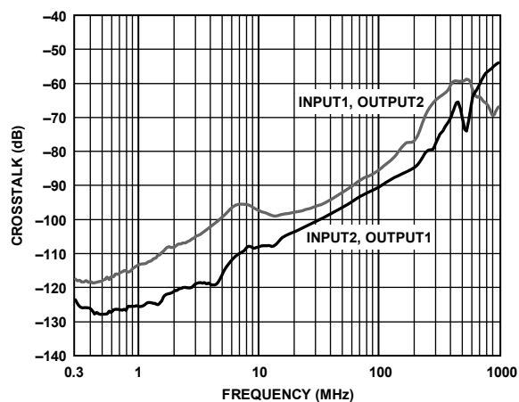
Figure 52. Crosstalk vs. Frequency for ADA4938-2
