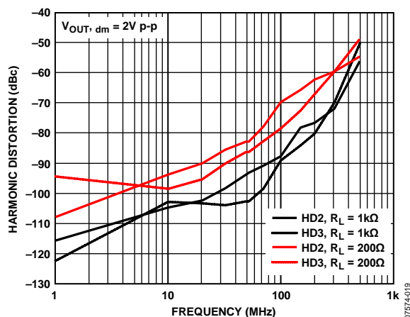
Figure 19. Harmonic Distortion vs. Frequency at Various Loads
