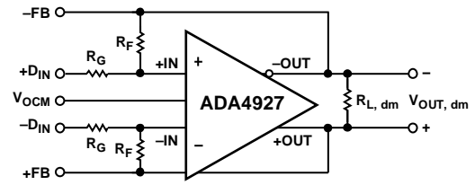
Figure 46. Circuit Definitions
