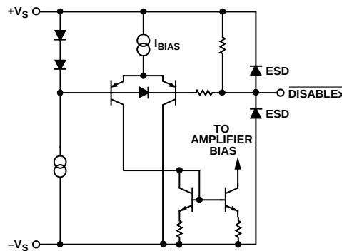
Figure 45. \overline{\text{DISABLEx}} Circuit
