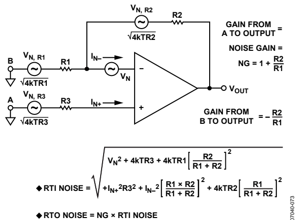
Figure 57. Operational Amplifier Noise Analysis Model
