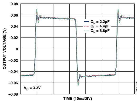
Figure 27. Small Signal Transient Response vs. Capacitive Load
