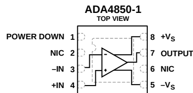
Figure 1. 8-Lead, 3 mm x 3 mm LFCSP
