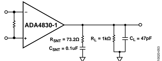
Figure 37. R-C Test Circuit
