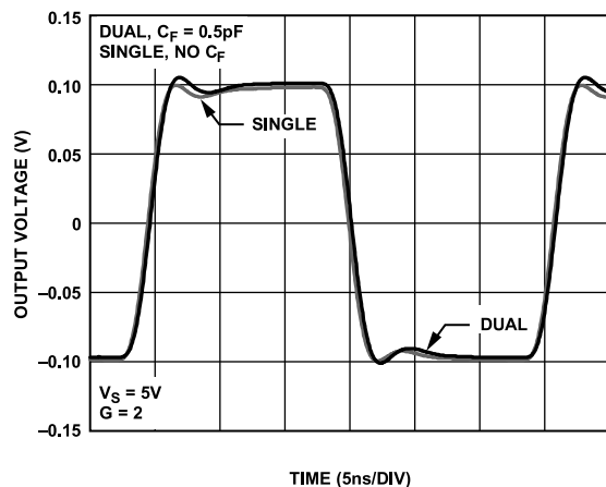
Figure 22. Small Signal Transient Response
