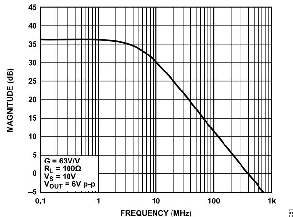
Figure 65. Photodiode Preamplifier Frequency Response
