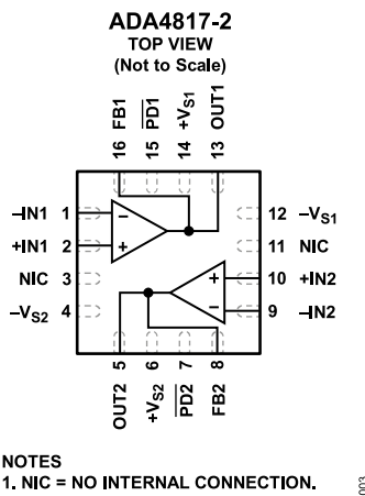
Figure 3. 16-Lead LFCSP (CP-16-20)
