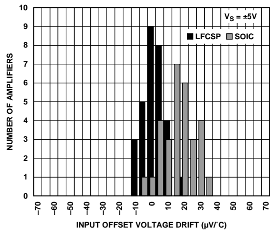
Figure 39. Input Offset Voltage Drift Histogram ( V_S = \pm 5\text{ V} )
