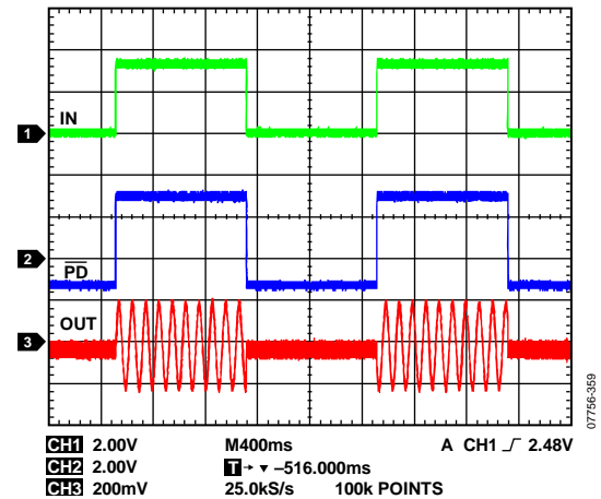
Figure 58. Power-Down Operation
