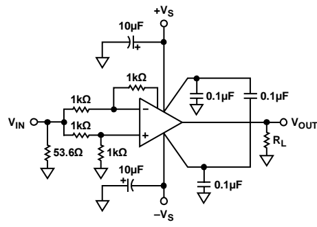
Figure 51. Common-Mode Rejection
