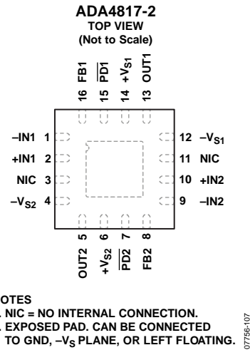
Figure 7. ADA4817-2 Pin Configuration (16-Lead LFCSP)
