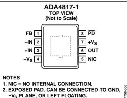
Figure 6. ADA4817-1 Pin Configuration (8-Lead SOIC)
