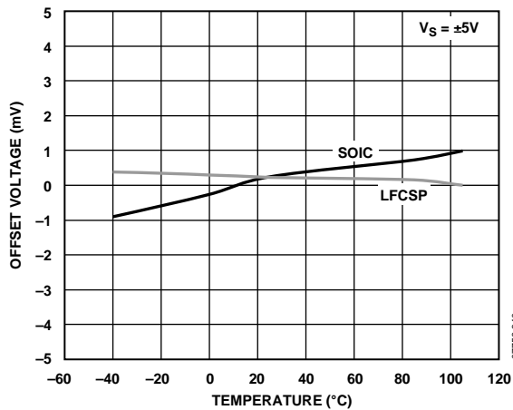
Figure 38. Offset Voltage vs. Temperature ( V_S = \pm 5\text{ V} )
