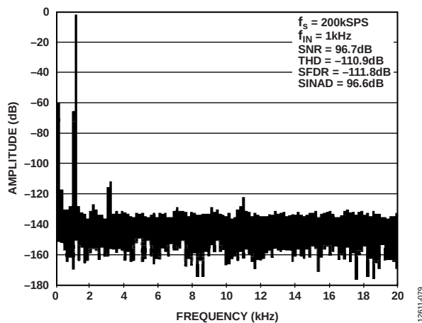
Figure 79. FFT for Driving a Differential Converter using Dynamic Power Scaling, -0.5 dBFS, On Time of 1.2 \mu\text{s} , for the Schematic Shown in Figure 74
