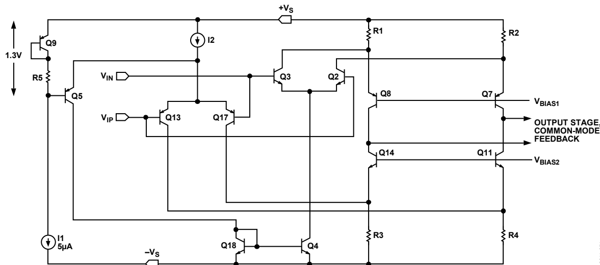
Figure 63. Simplified Schematic
