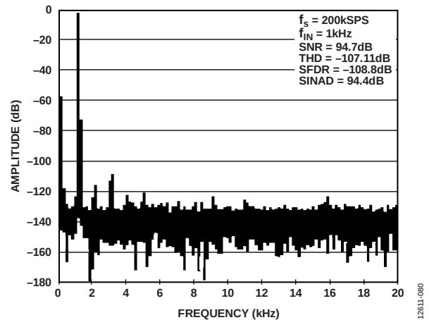
Figure 81. FFT for Driving a Single-Ended to Differential Converter Using Dynamic Power Scaling, -0.5 dBFS, On Time of 4 \mu\text{s} , for the Schematic Shown in Figure 76
