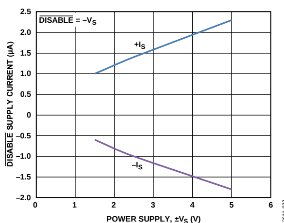
Figure 27. DISABLE Supply Current vs. Power Supply, ±V S
