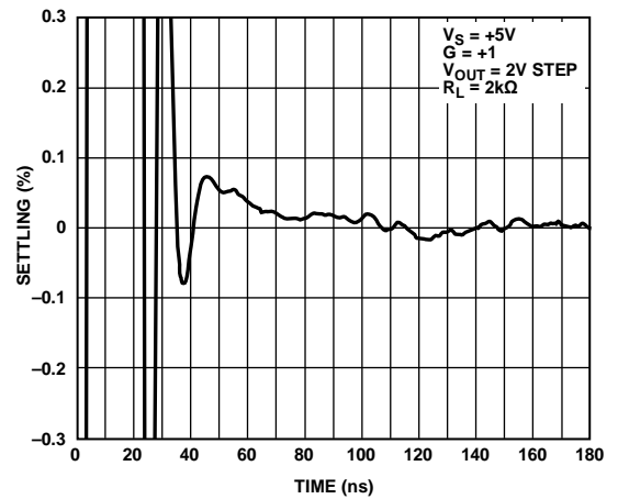
Figure 22. Settling Time to 0.1%
