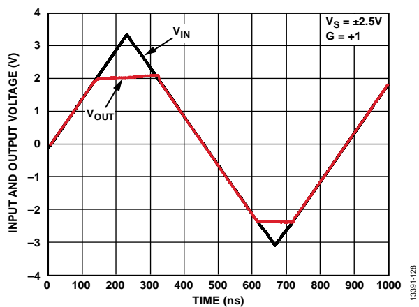
Figure 30. Input Overdrive Recovery Time
