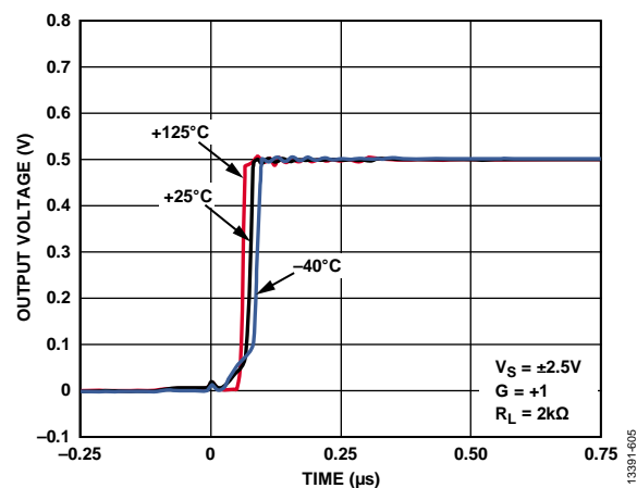
Figure 34. Turn-On Response Time from Sleep for Various Temperatures (See Figure 50)
