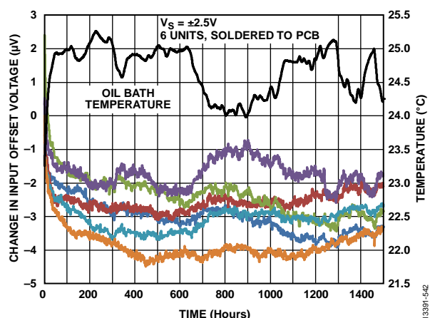
Figure 43. Long-Term V_{OS} Drift
