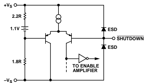
Figure 54. Shutdown/Sleep Equivalent Circuit
