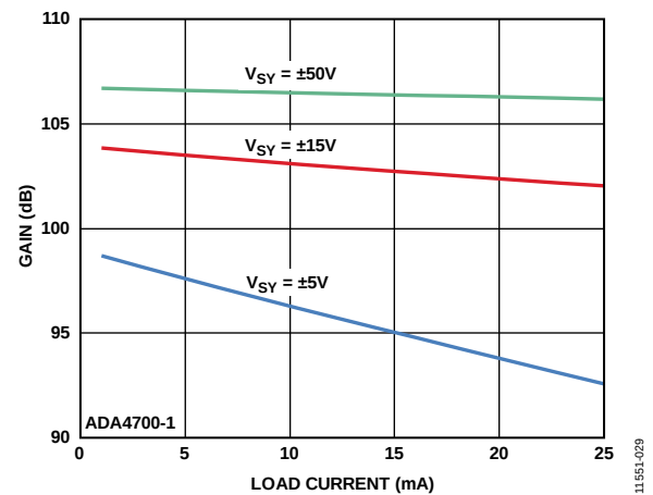
Figure 25. Open-Loop Gain vs. Load Current for Various Supply Voltages
