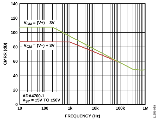
Figure 37. Common-Mode Rejection Ratio (CMRR) vs. Frequency, V_{SY} = \pm 5V to \pm 50V
