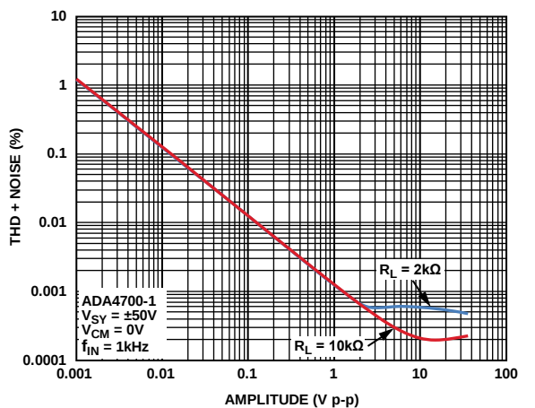
Figure 33. Total Harmonic Distortion + Noise (THD + Noise) vs. Amplitude, V_{SY} = \pm 50\text{V}
