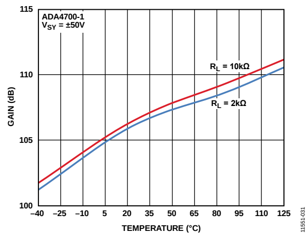
Figure 26. Open-Loop Gain vs. Temperature for Various Load Resistances, V_{SY} = \pm 50\text{ V}
