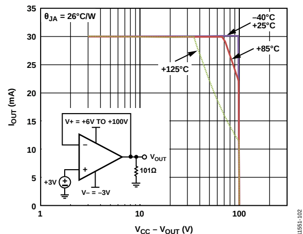
Figure 59. Safe Operating Area with \theta_{JA} = 26^\circ\text{C/W}
