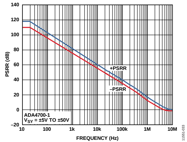
Figure 38. Power Supply Rejection Ratio (PSRR) vs. Frequency, V_{SY} = \pm 5V to \pm 50V
