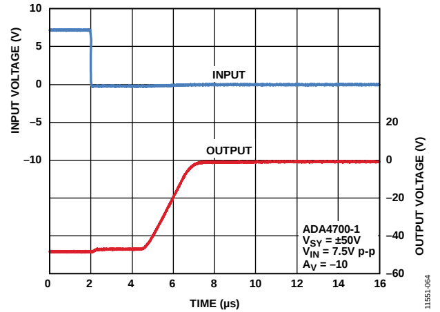
Figure 45. Negative Output Overload Recovery, V_{SY} = \pm 50V
