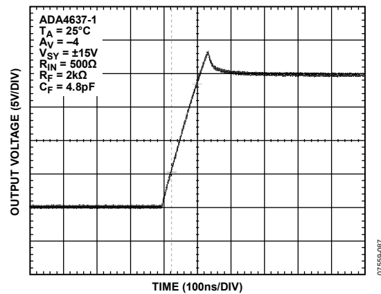
Figure 45. Slew Rate Rising
