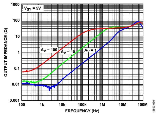
Figure 33. Z_{OUT} vs. Frequency, V_{SY} = 5V
