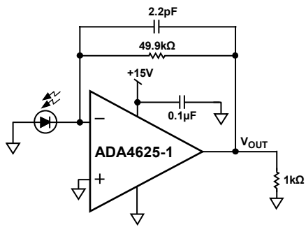
Figure 101. Single-Supply TIA Circuit Using the ADA4625-1
