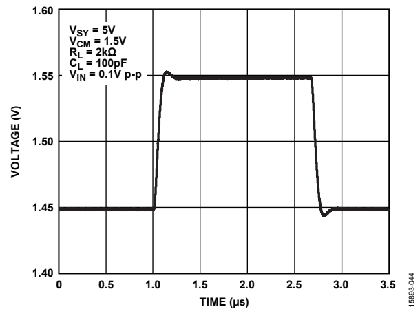
Figure 51. Small Signal Transient Response, A_V = -1 , V_{SY} = 5V
