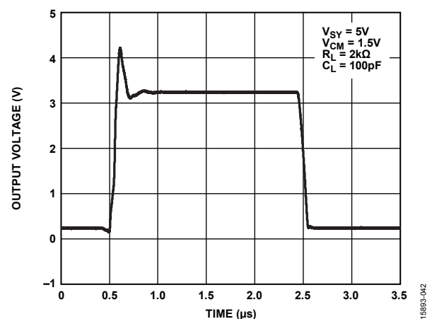
Figure 46. Large Signal Transient Response, A_V = -1 , V_{SV} = 5V
