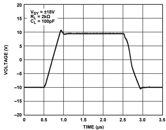
Figure 43. Large Signal Transient Response, A_V = -1 , V_{SV} = \pm 18V
