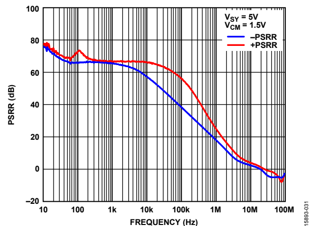
Figure 34. PSRR vs. Frequency, V_{SY} = 5V
