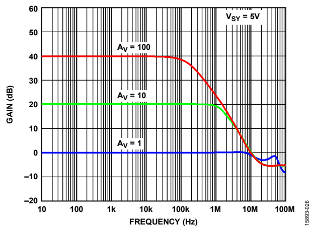
Figure 32. Gain vs. Frequency for Various Closed-Loop Gains, V_{SY} = 5V
