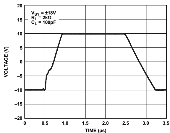
Figure 42. Large Signal Transient Response, A_V = +1 , V_{SV} = \pm 18V
