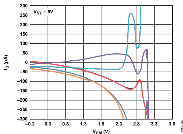
Figure 20. I_B vs. V_{CM} , V_{SY} = 5 V
