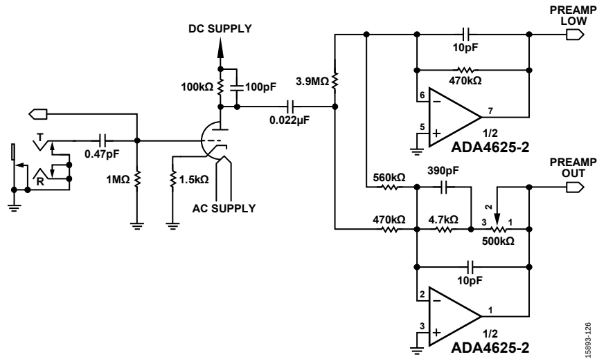
Figure 111. Guitar Preamplifier
