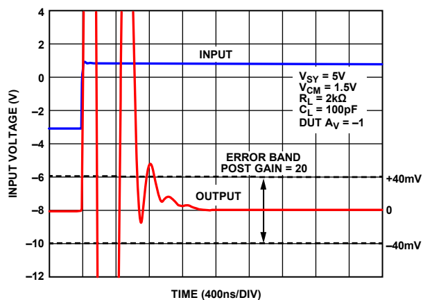
Figure 69. ADA4625-2 Positive Settling Time to 0.1%, V_{SY} = 5V
