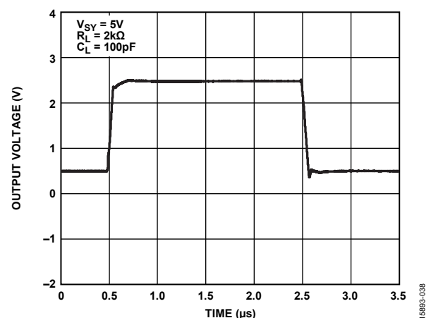
Figure 45. Large Signal Transient Response, A_V = +1 , V_{SV} = 5V
