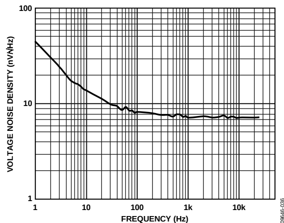
Figure 41. Voltage Noise Density vs. Frequency, V_{SY} = \pm 15\text{ V}
