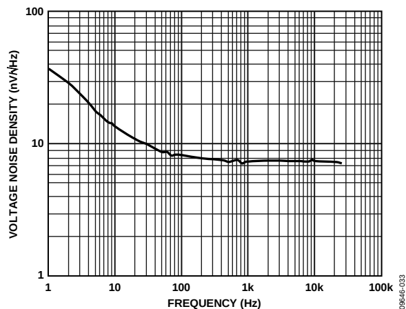
Figure 39. Voltage Noise Density vs. Frequency, V_{SY} = \pm 5\text{ V}
