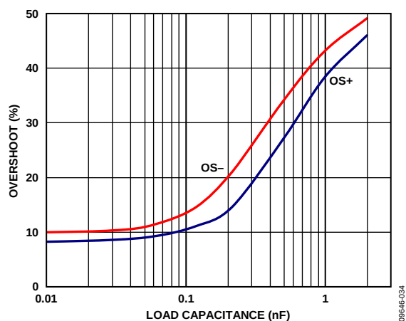
Figure 40. Overshoot vs. Load Capacitance, V_{SY} = \pm 5\text{ V} , A_V = 1 , R_L = 2\text{ k}\Omega , V_{IN} = 100\text{ mV p-p}
