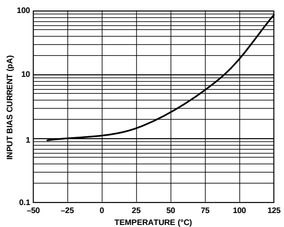
Figure 17. Input Bias Current vs. Temperature, V_{SY} = \pm 5\text{ V}
