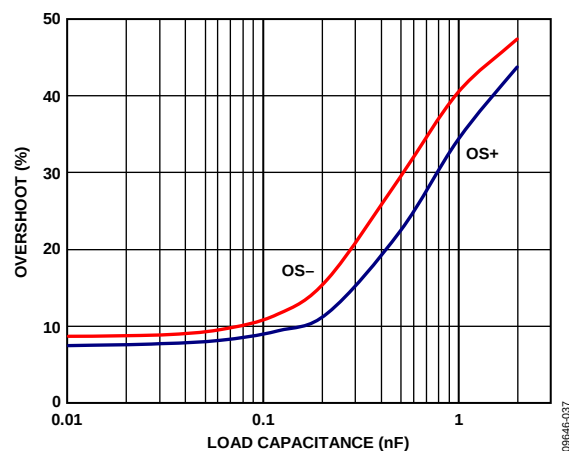
Figure 42. Overshoot vs. Load Capacitance, V_{SY} = \pm 15\text{ V} , A_V = 1 , R_L = 2\text{ k}\Omega , V_{IN} = 100\text{ mV p-p}
