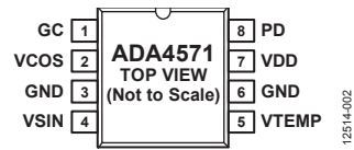
Figure 2. Pin Configuration
