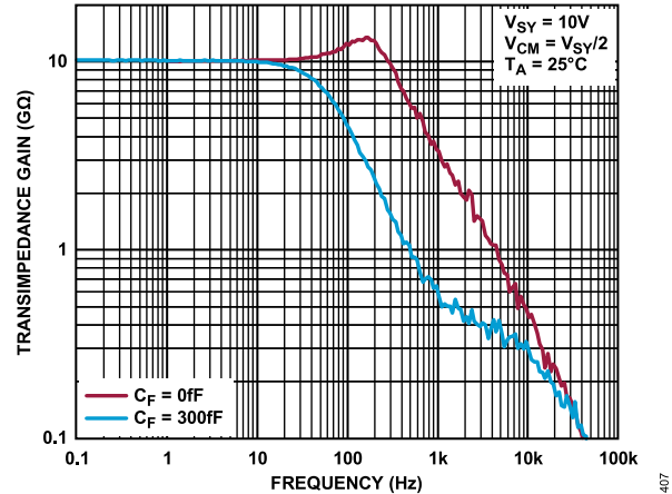
Figure 129. Transimpedance Gain vs. Frequency
