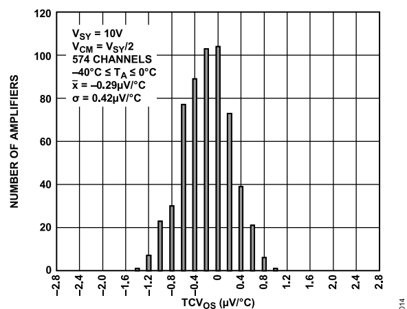
Figure 11. Input Offset Voltage Drift Distribution, -40^{\circ}C \leq T_A \leq 0^{\circ}C , V_{SY} = 10 V
