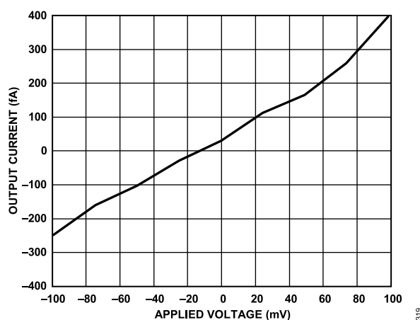
Figure 114. Current to Voltage Response of RMA Contaminated Insulation
