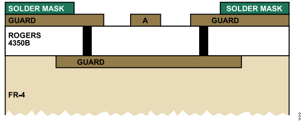
Figure 123. Layout Cross Section with Guard Plane
