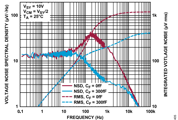
Figure 131. RTO Noise Spectral Density (25°C)
