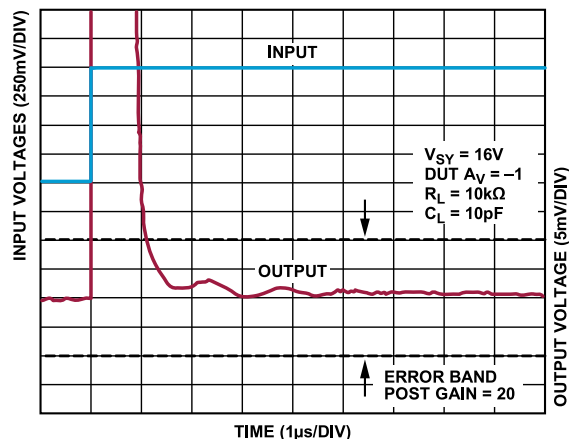
Figure 78. Positive Settling Time to 0.1%, V_{SY} = 16\text{ V}
