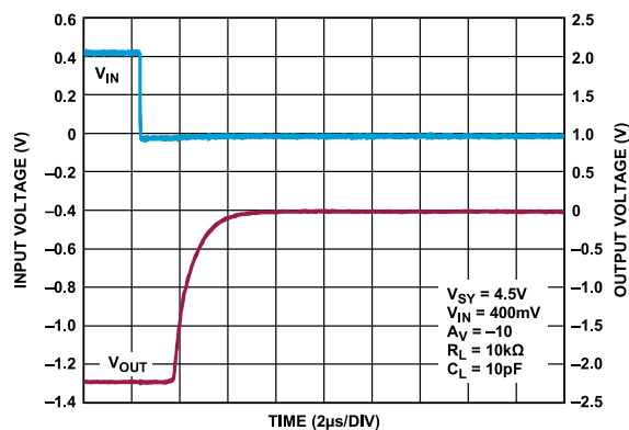
Figure 70. Negative Overload Recovery, V_{SY} = 4.5\text{ V}
