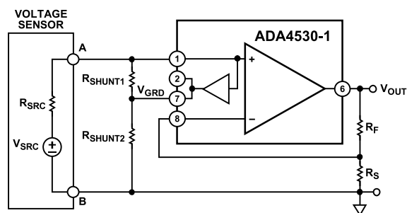
Figure 107. Voltage Buffer Circuit with Guard
