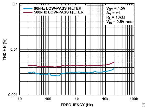
Figure 79. THD + N vs. Frequency, V_{SY} = 4.5\text{ V}
