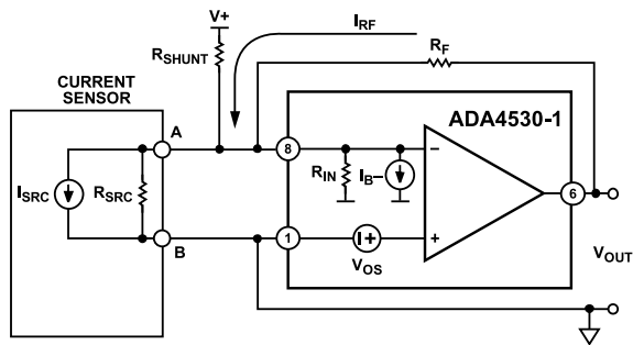
Figure 106. TIA Circuit
