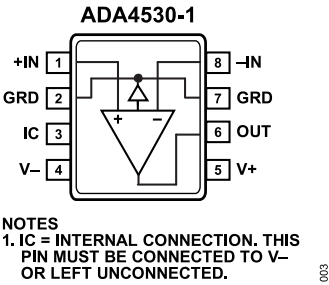
Figure 3. Pin Configuration
