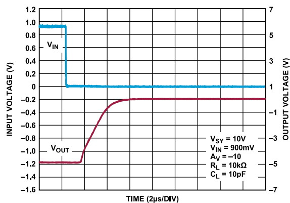
Figure 71. Negative Overload Recovery, V_{SY} = 10\text{ V}
