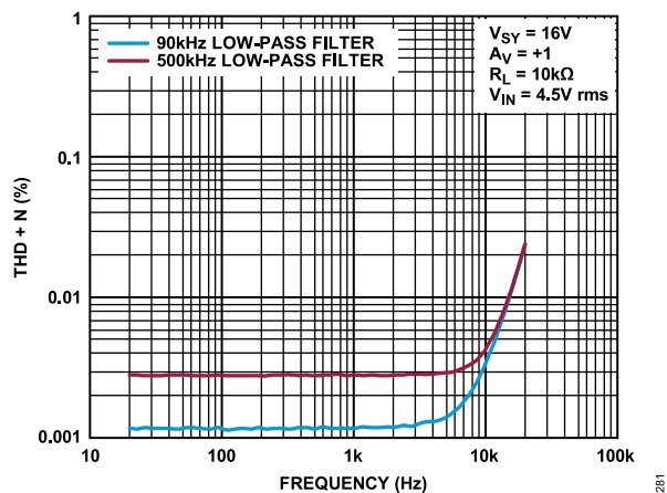
Figure 81. THD + N vs. Frequency, V_{SY} = 16\text{ V}
