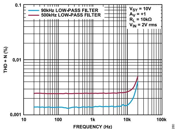
Figure 80. THD + N vs. Frequency, V_{SY} = 10\text{ V}
