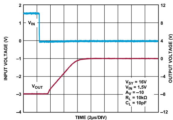
Figure 72. Negative Overload Recovery, V_{SY} = 16\text{ V}
