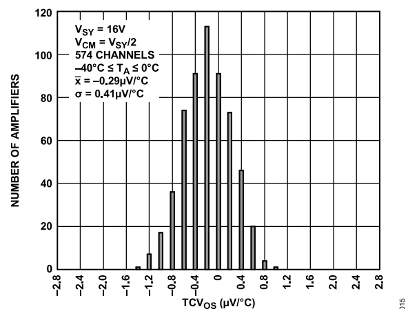
Figure 12. Input Offset Voltage Drift Distribution, -40^{\circ}C \leq T_A \leq 0^{\circ}C , V_{SY} = 16 V
