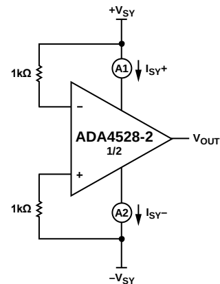
Figure 70. Comparator A
