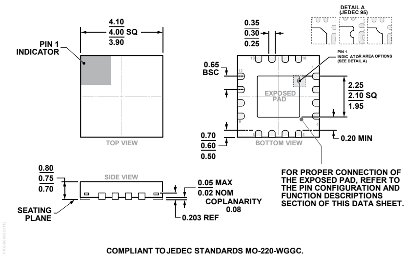
Figure 23. 16-Lead Lead Frame Chip Scale Package [LFCSP] 4 mm × 4 mm Body and 0.75 mm Package Height (CP-16-23) Dimensions shown in millimeters
