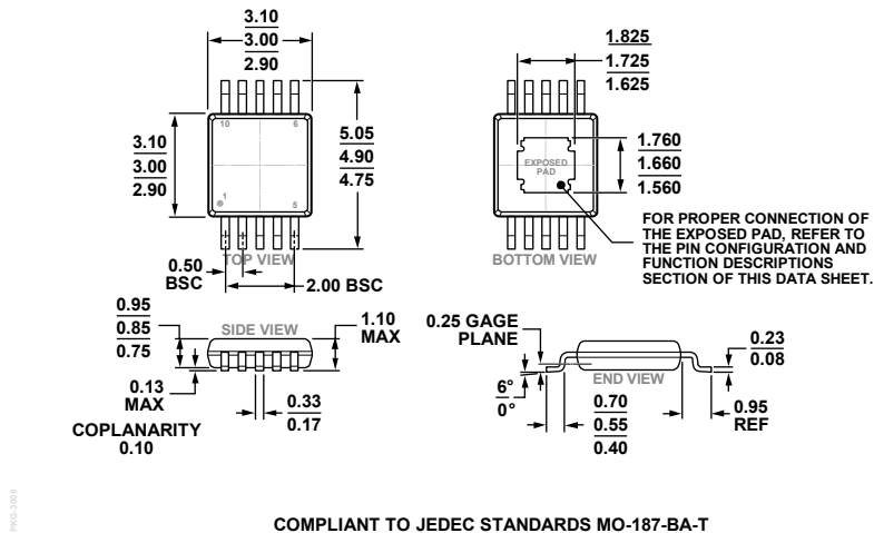
Figure 22. 10-Lead Mini Small Outline Package with Exposed Pad [MINI_SO_EP] (RH-10-1) Dimensions shown in millimeters
