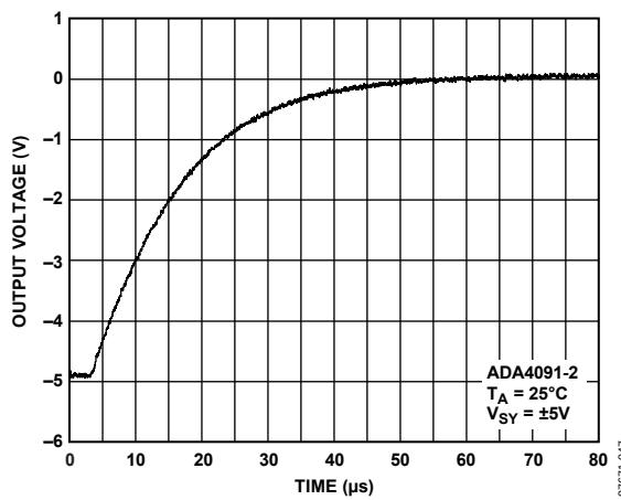
Figure 28. Negative Overload Recovery
