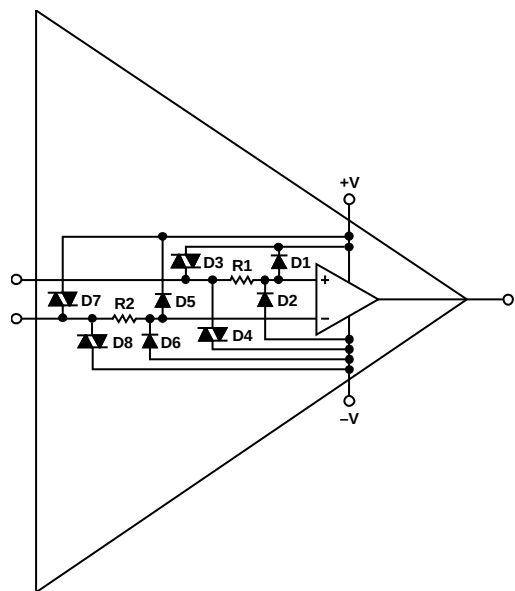
Figure 48. Complete Input Protection Network
