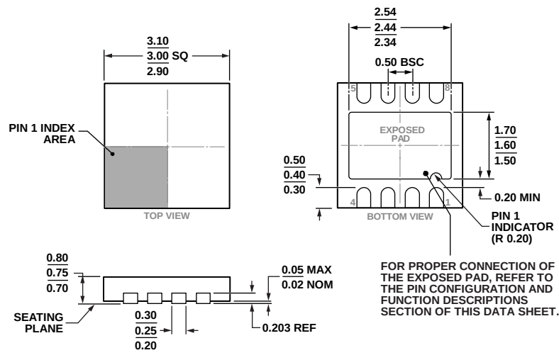
Figure 51. 8-Lead Lead Frame Chip Scale Package [LFCSP] 3 mm × 3 mm Body and 0.75 mm Package Height (CP-8-21)
