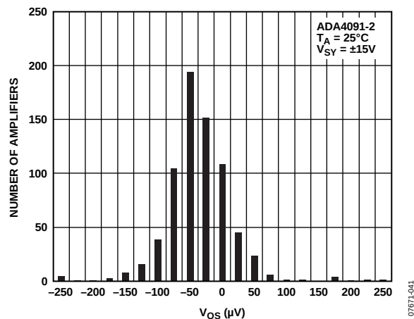
Figure 29. Input Offset Voltage Distribution
