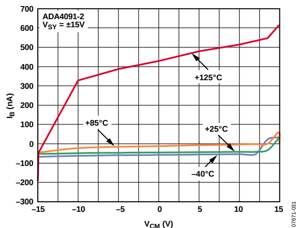
Figure 31. Input Bias Current vs. Common-Mode Voltage
