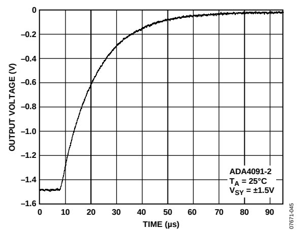
Figure 16. Negative Overload Recovery
