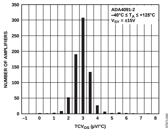
Figure 30. TCV_{OS} Distribution
