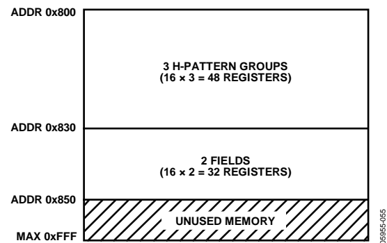
Figure 55. Example Register Configuration
