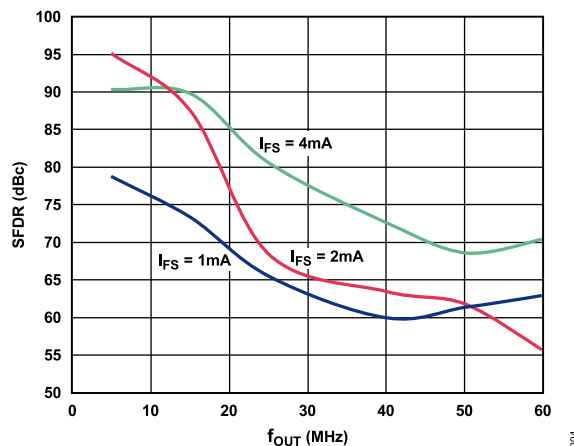
Figure 7. Third Harmonic Distortion vs. f_{OUT} Over Full-Scale Current, f_{DAC} = 125 MHz, 1x, Digital Scale = 0 dBFS, TXVDD = 3.3 V
