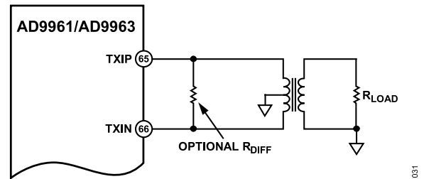
Figure 61. Differential Output Using a Transformer
