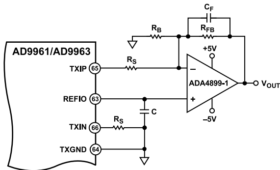
Figure 63. Single-Supply Single-Ended Buffer
