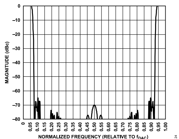
Figure 51. Digital Filter Transfer Function for 8 \times Interpolation
