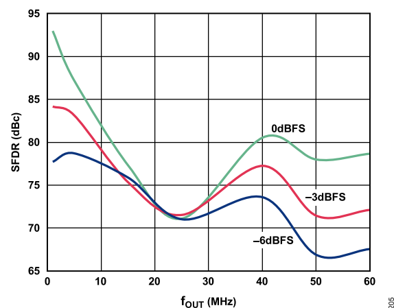
Figure 8. Second Harmonic Distortion vs. f_{OUT} Over Digital Scale, f_{DAC} = 125 MHz, 1x, Full-Scale Current = 2 mA, TXVDD = 1.8 V
