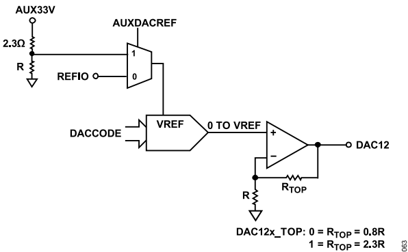
Figure 91. Simplified Schematic of the 12-Bit Auxiliary DAC
