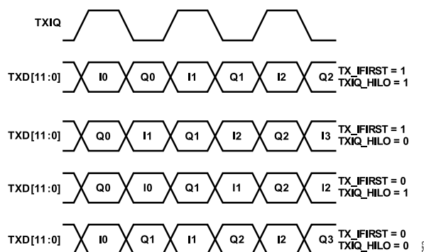
Figure 80. Transmit Path Data Pairing Options
