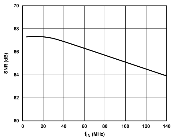
Figure 30. AD9963 1.8 V CMOS IADC, 100 MSPS Single Tone AC
