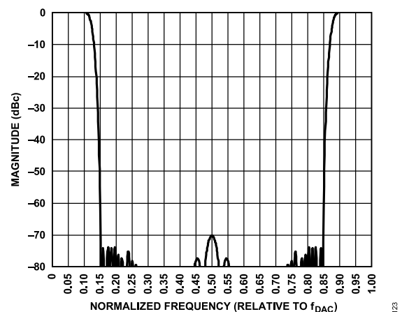
Figure 50. Digital Filter Transfer Function for 4 \times Interpolation
