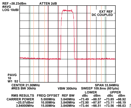
Figure 17. One-Carrier W-CDMA ACLR Performance, IF = ~21 MHz
