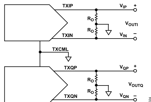
Figure 58. Basic Transmit DAC Output Circuit
