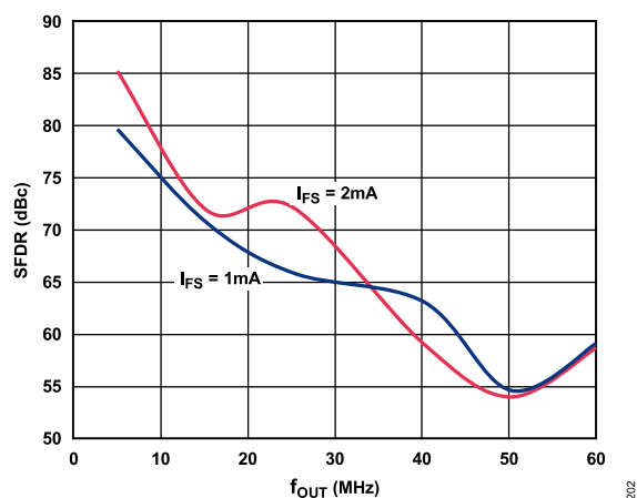
Figure 5. Third Harmonic Distortion vs. f_{OUT} Over Full-Scale Current, f_{DAC} = 125 MHz, 1x, Digital Scale = 0 dBFS, TXVDD = 1.8 V
