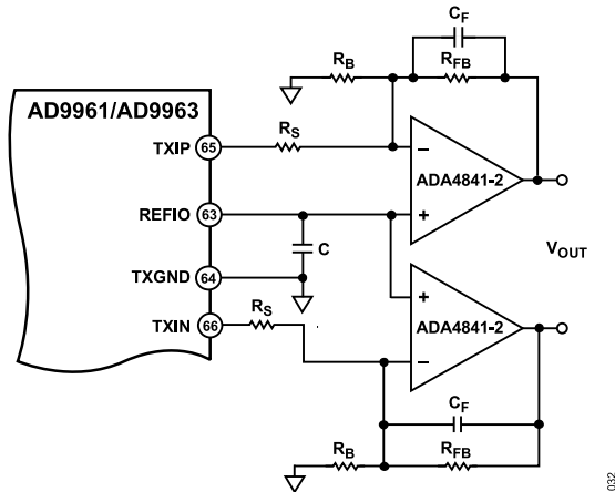
Figure 62. Single-Supply Differential Buffer
