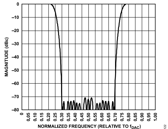
Figure 49. Digital Filter Transfer Function for 2 \times Interpolation
