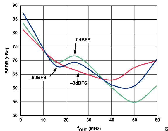
Figure 9. Third Harmonic Distortion vs. f_{OUT} Over Digital Scale, f_{DAC} = 125 MHz, 1x, Full-Scale Current = 2 mA, TXVDD = 1.8 V
