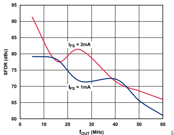
Figure 4. Second Harmonic Distortion vs. f_{OUT} Over Full-Scale Current, f_{DAC} = 125 MHz, 1x, Digital Scale = 0 dBFS, TXVDD = 1.8 V
