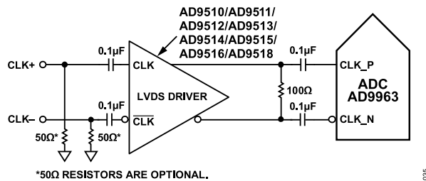
Figure 66. Differential LVDS Sample Clock
