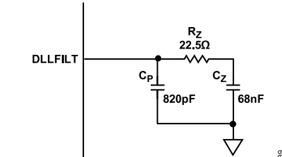
Figure 71. Recommended DLL Loop Filter
