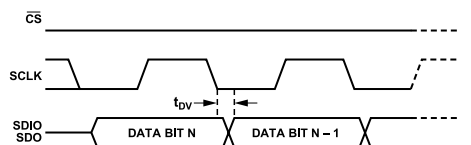
Figure 36. Timing Diagram for Serial Control Port Register Read
