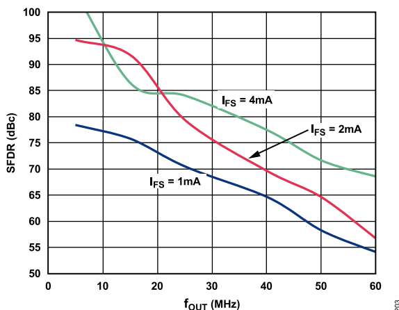
Figure 6. Second Harmonic Distortion vs. f_{OUT} Over Full-Scale Current, f_{DAC} = 125 MHz, 1x, Digital Scale = 0 dBFS, TXVDD = 3.3 V
