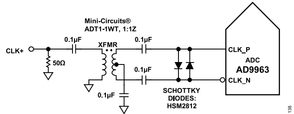
Figure 69. Transformer Coupled Clock
