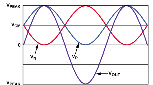
Figure 59. Voltage Output Waveforms
