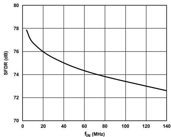
Figure 29. AD9963 100 MSPS Single Tone AC
