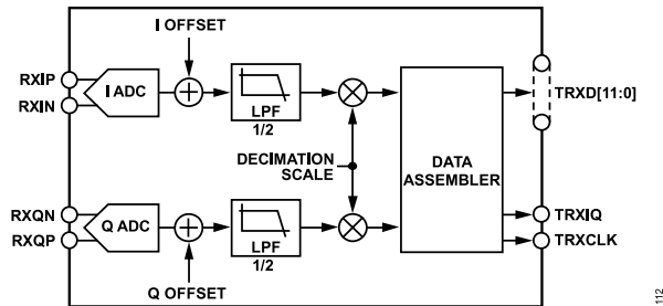
Figure 39. Receive Path Block Diagram
