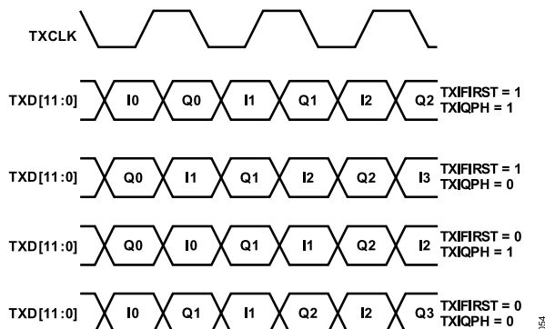
Figure 82. Transmit Path Timing Modes (DDR Mode)
