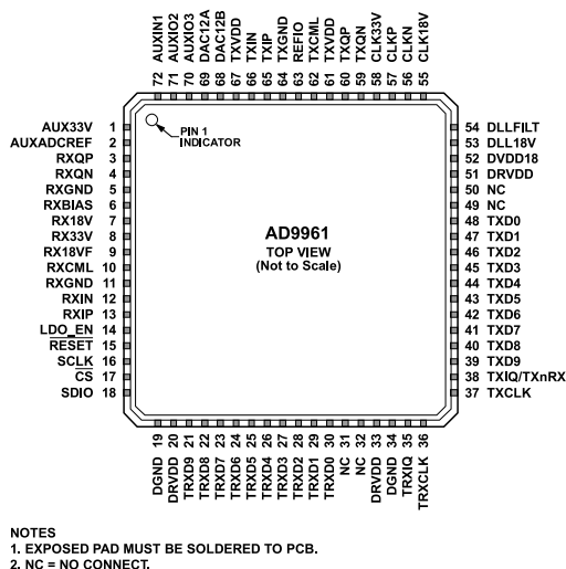
Figure 2. AD9961 Pin Configuration
