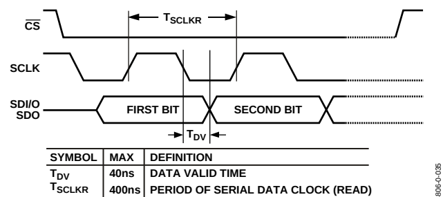
Figure 34. Timing Diagram for Data Read to AD9956
