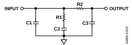
Figure 2. Generic Loop Filter
