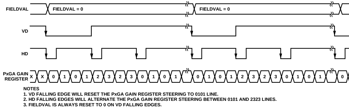
Figure 33. PxGA Color Steering—Progressive Mode
