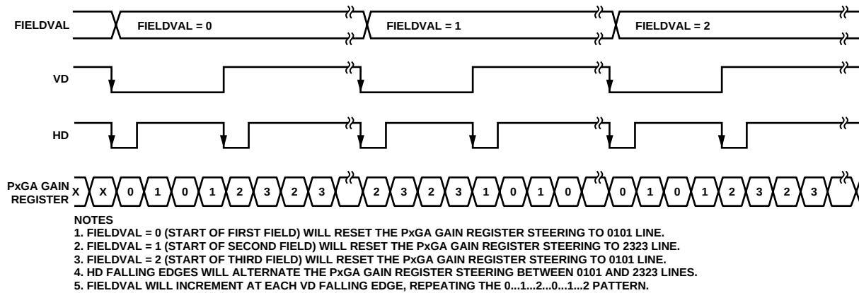
Figure 35. PxGA Color Steering—Three-Field Mode
