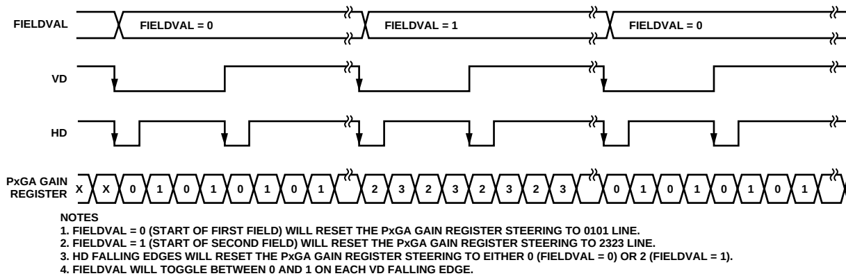
Figure 34. PxGA Color Steering—Interlaced Mode
