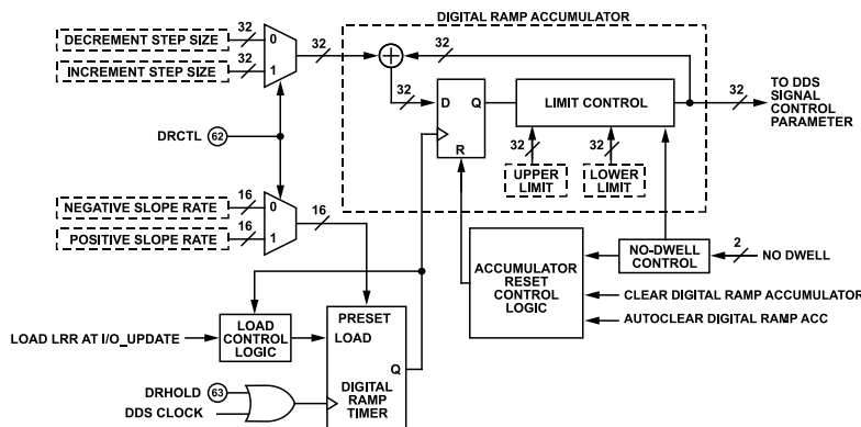
Figure 37. Digital Ramp Generator Detail
