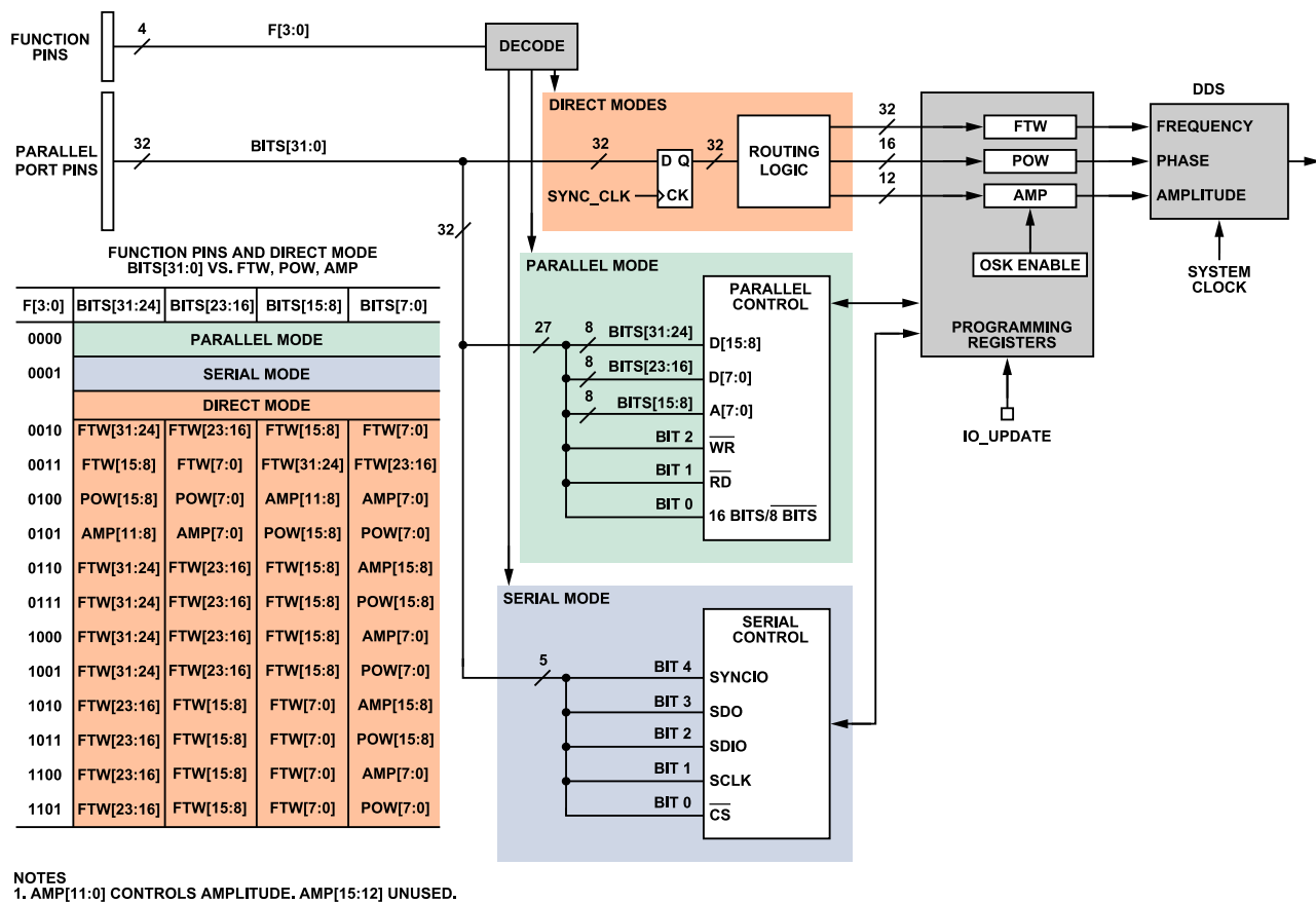
Figure 41. Parallel Port Block Diagram
