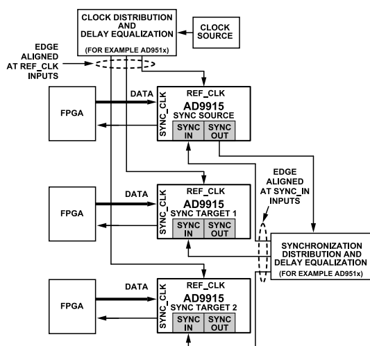
Figure 49. Configuration of Multiple Devices to Be Synchronized
