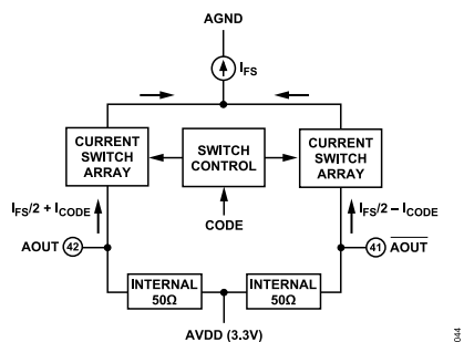
Figure 26. DAC Output
