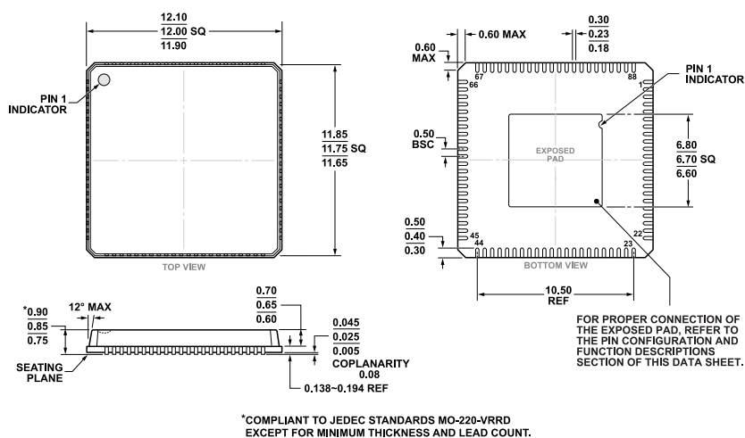
Figure 50. 88-Lead Lead Frame Chip Scale Package [LFCSP_VQ] 12 mm x 12 mm Body, Very Thin Quad (CP-88-5) Dimensions shown in millimeters
