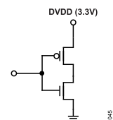
Figure 28. CMOS Input
