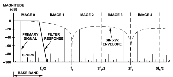
Figure 31. DAC Spectrum vs. Reconstruction Filter Response
