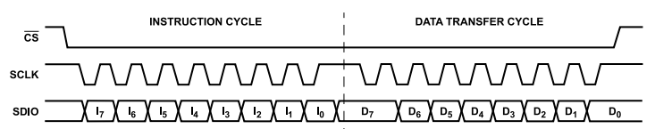
Figure 44. Serial Port Write Timing, Clock Stall High
