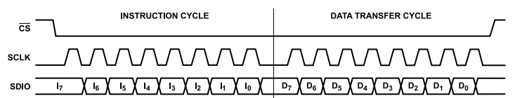
Figure 42. Serial Port Write Timing, Clock Stall Low
