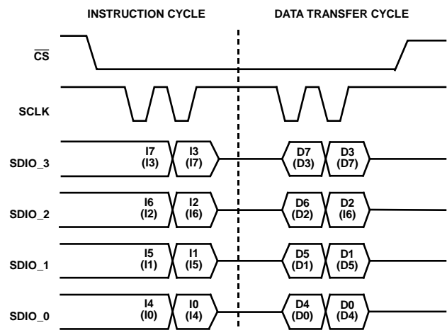
Figure 56. 4-Bit Mode Read Timing—Clock Stall High
