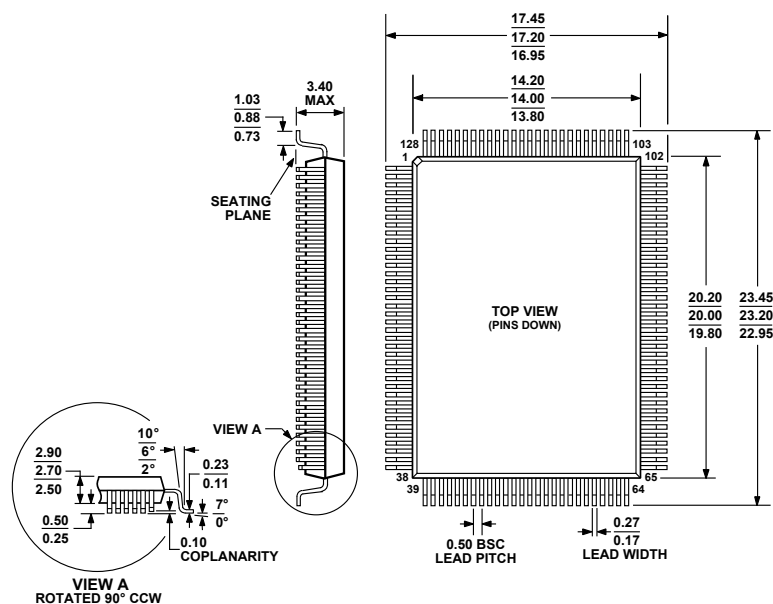
Figure 28. 128-Lead Metric Quad Flat Package [MQFP] (S-128-1)
