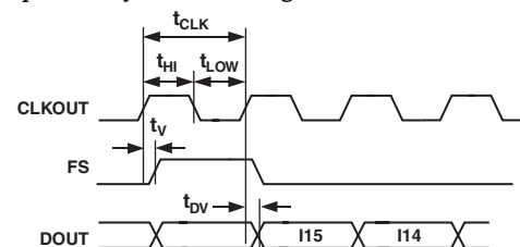
Figure 3b. Timing Parameters for SSI Timing*
