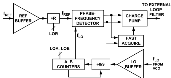
Figure 39. LO Synthesizer
