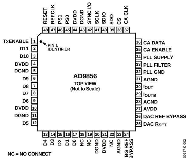
Figure 2. Pin Configuration
