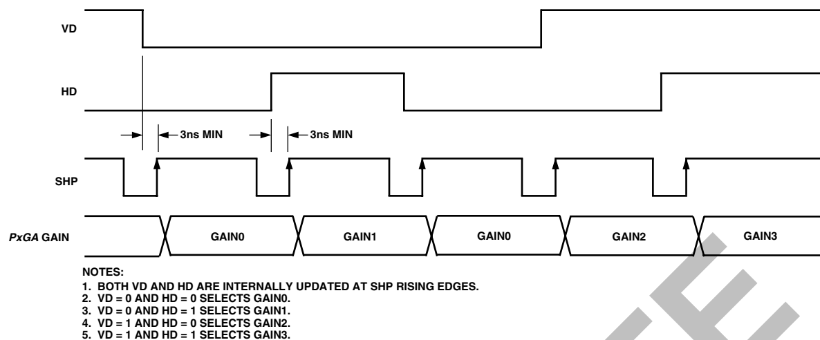
Figure 20. PxGA Mode 7 (User-Specified) Detailed Timing
