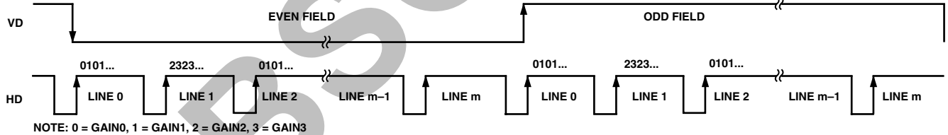
Figure 10. PxGA Mode 2 (Interlace) Frame/Line Gain Register Sequence
