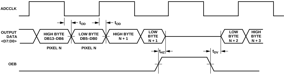
Figure 7. Digital Output Data Timing
