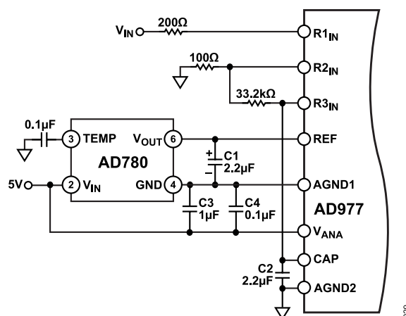
Figure 19. AD780 External Reference to AD977 Configured for \pm 10 V Input Range
