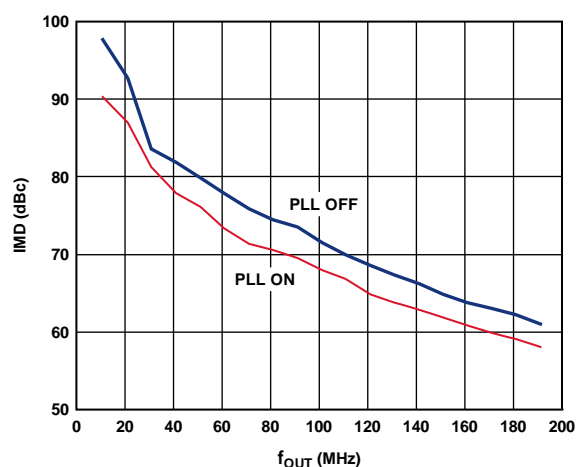
Figure 22. AD9779A Third-Order IMD vs. f_{OUT} , 4× Interpolation, f_{DATA} = 100 MSPS, PLL On/Off
