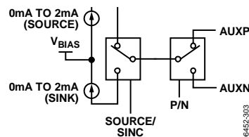
Figure 78. Auxiliary DAC Source/Sink for AD9776A/AD9778A/AD97779A
