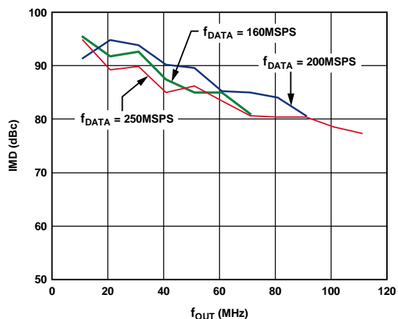
Figure 18. AD9779A Third-Order IMD vs. f_{OUT} , 1× Interpolation
