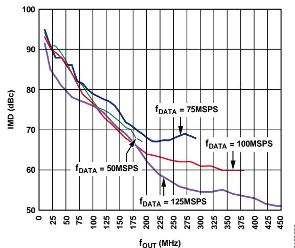
Figure 21. AD9779A Third-Order IMD vs. f_{OUT} , 8× Interpolation
